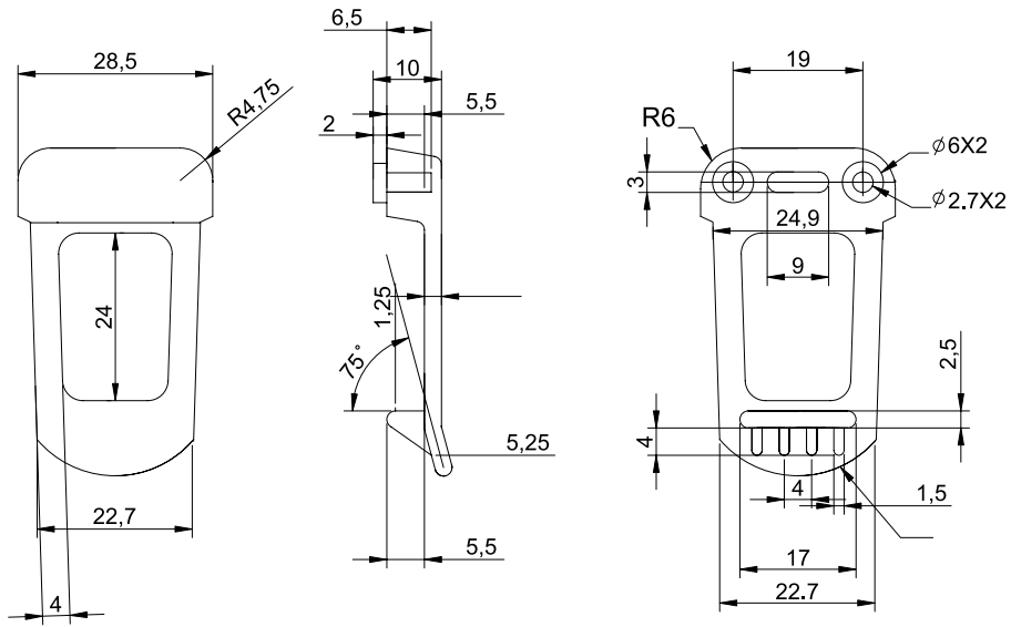
G909 Clip
